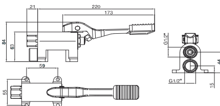
ART.02061 Torneira Pedal Horizontal
